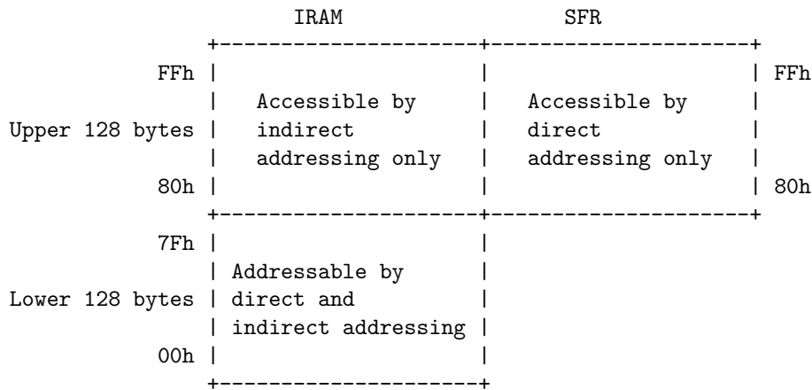
nRF24E1 Internal Data Memory Structure Overview:
